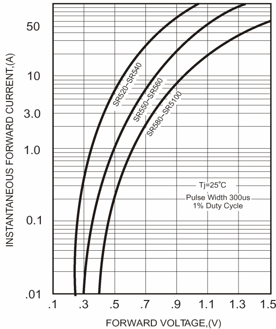
FIG.2-TYPICAL FORWARD CHARACTERISTICS
